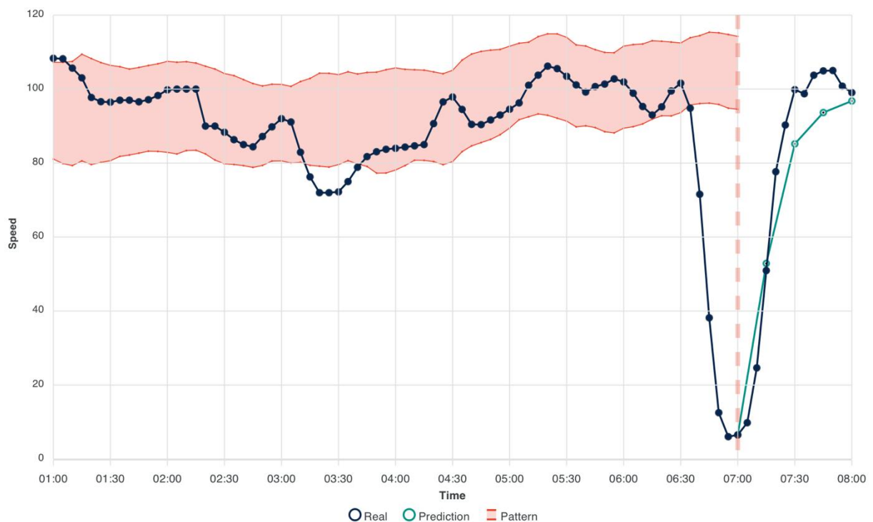
Figure 3 Illustration of Aimsun's Incident Detection Module (IDM) traffic flow monitoring
